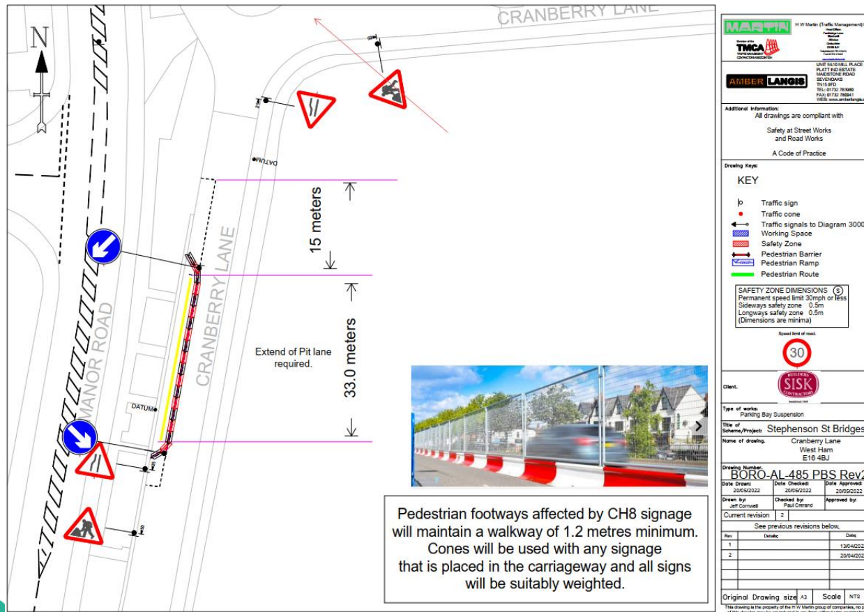
Traffic management plan for car park closure / suspension
