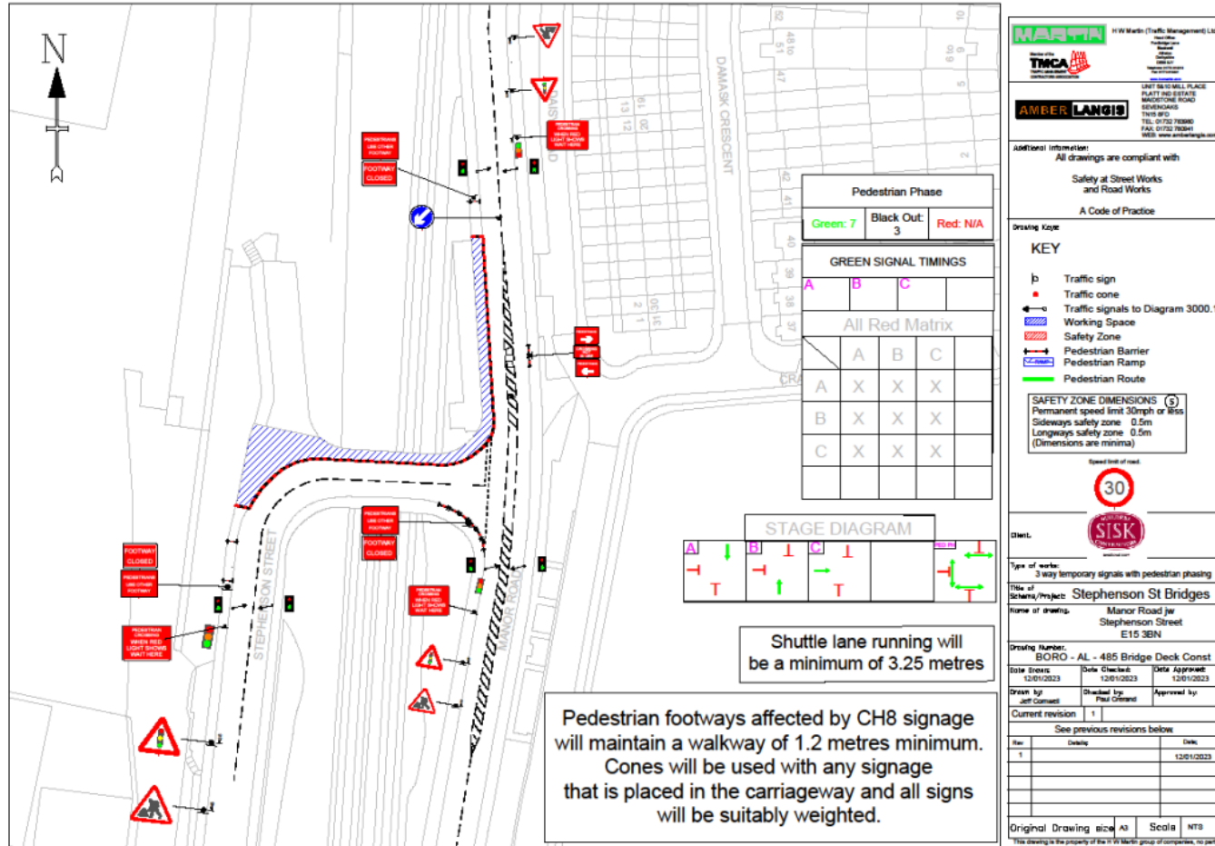
Traffic management plan for footpath closure
